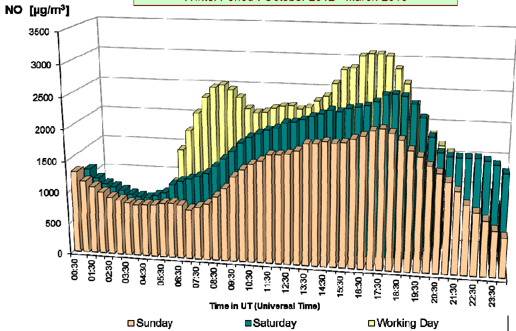
NO at 41LEB2 - TUNNEL LEOPOLD II - Basilica Average SUNDAY, SATURDAY and WORKING DAY Winter Period : October 2012 - March 2013
