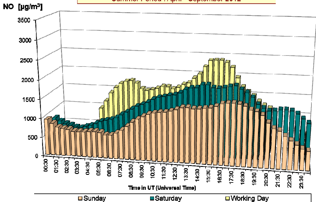
NO at 41LEB2 - TUNNEL LEOPOLD II - Basilica Average SUNDAY, SATURDAY and WORKING DAY Summer Period : April - September 2012
