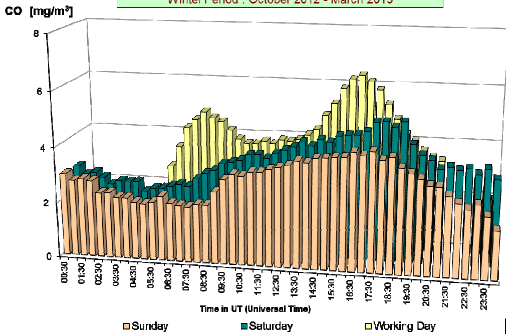
CO at 41LEB2 - TUNNEL LEOPOLD II - Basilica Average SUNDAY, SATURDAY and WORKING DAY Winter Period : October 2012 - March 2013
