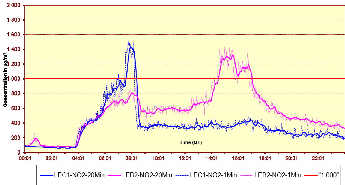
NO 2 - 20-Minutes Average - Tunnel Leopold II Friday 14 September 2012
