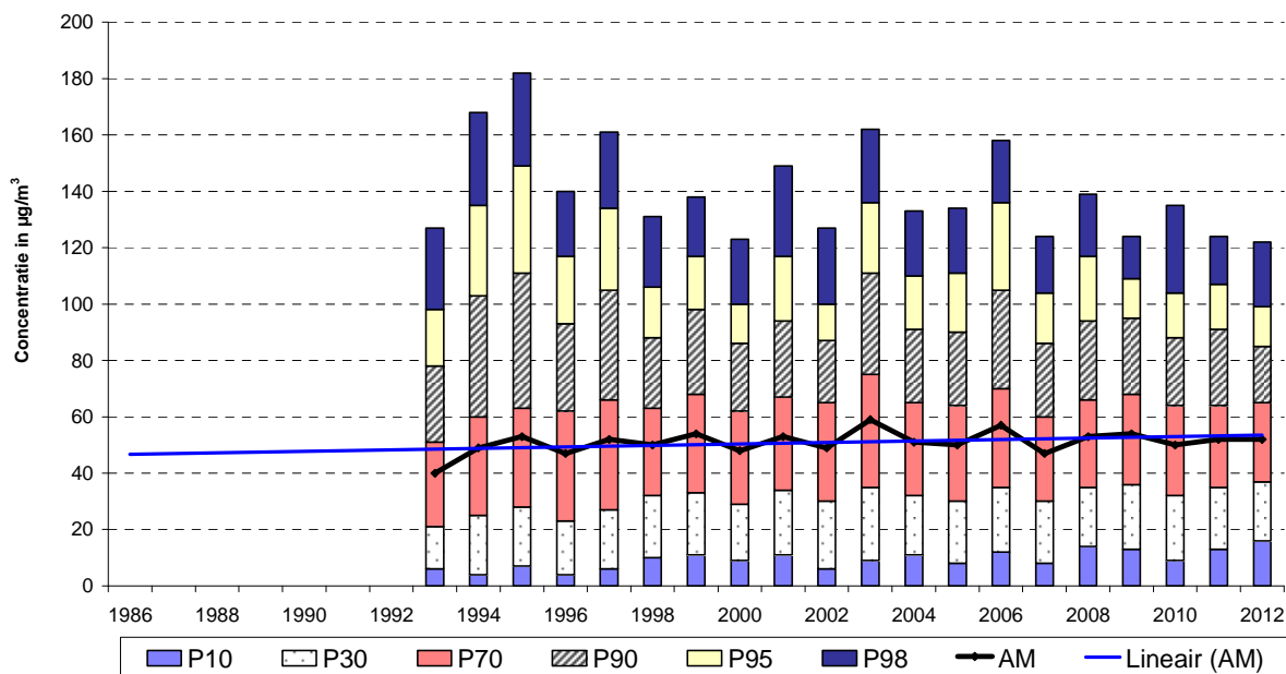
Fig. 34 : Evolutive O 3 -uurwaarden te St.-Ag.-Berchem (1993-2012) Zomerperiode "april – september"
